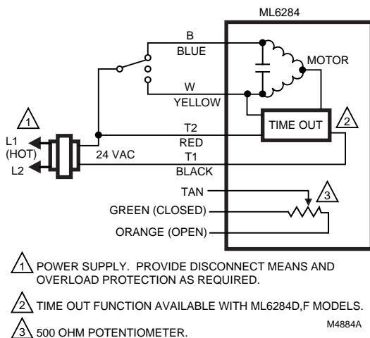
Fig. 6. ML6284D,F typical wiring diagram.
