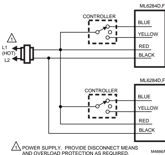
Fig. 9. Common transformer with two controller outputs and two ML6284D,F actuators.
