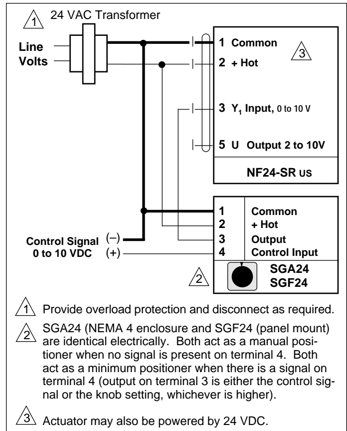
Minimum position control of NF24-SR us from a voltage signal and through a SGA24/SGF24 positioner.
