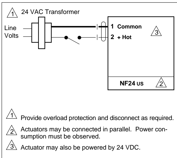
On-off wiring for NF24 us
