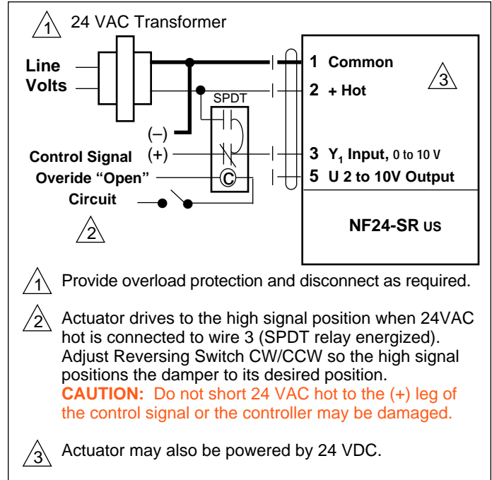
Override open of a NF24-SR us Both the override closed and the override open circuit can be combined on one actuator. Wire the relay contacts in series. Determine which signal has the highest precedence and connect that relay electrically closest to the actuator.
