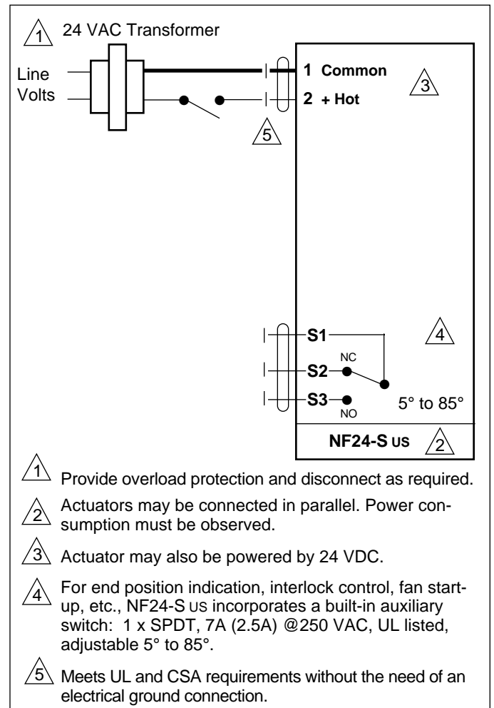
On-off wiring for NF24-S us
