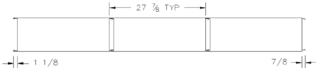
Typical Insulated Oven Panel Joint
